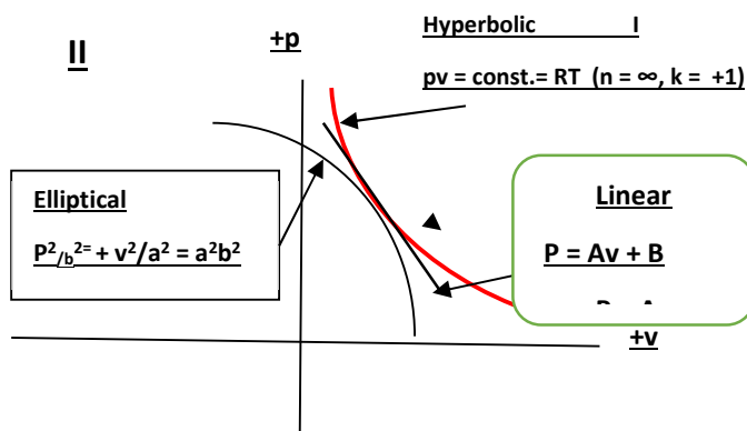
Fig. 1: Three Equations State in Quadrant 1 at a Tangent Point: Hyperbolic for Visible Matter, Elliptical for the Dark Matter, Tangent Linear for Compressive Electromagnetic Photons
