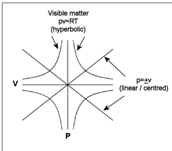
Figure 2. The Universal, Centered, Linear, State which uniquely and universally intersects with the hyperbolic, visible matter states in Quadrant 1;( Note: the universal intersctions with the elliptical and the tangent, linear states (Fig. 1) are similarly depictable)
